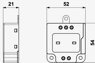
Product dimensions
