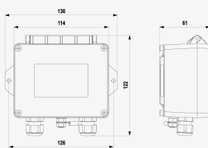
Product dimensions
