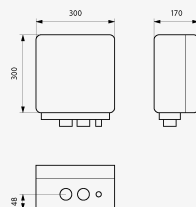
Product dimensions
