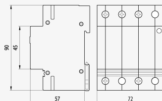
Product dimensions
