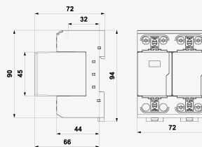
Product dimensions
