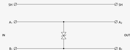
Basic circuit diagram
