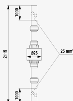
Product dimensions
