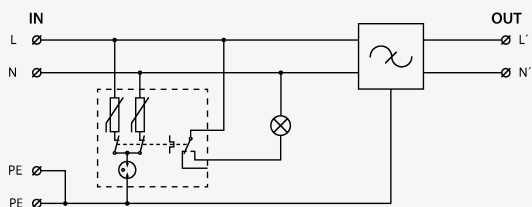
Basic circuit diagram
