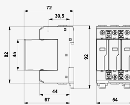
Product dimensions
