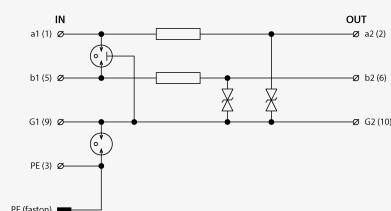
Basic circuit diagram
